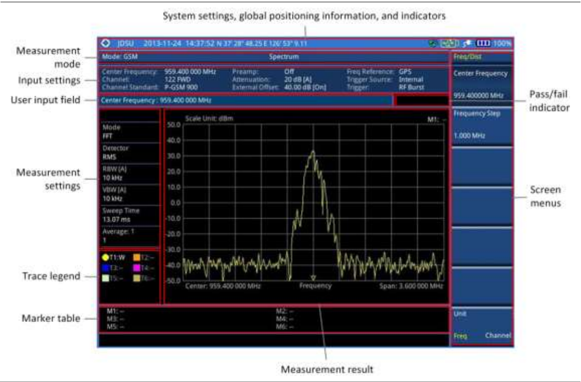
Figure 41 GSM signal analyzer measurement screen
