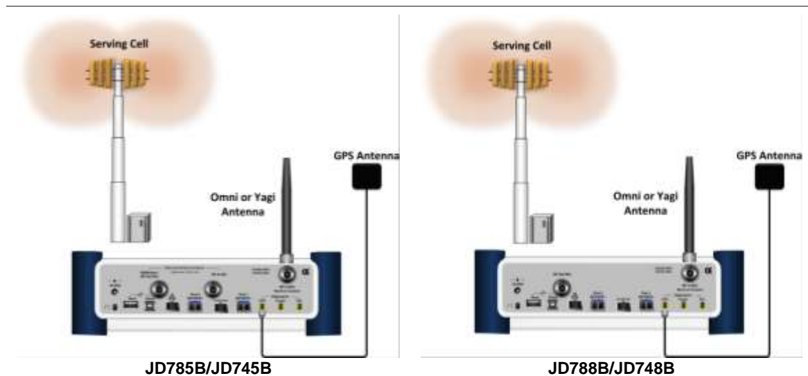
Figure 63 OTA connection
