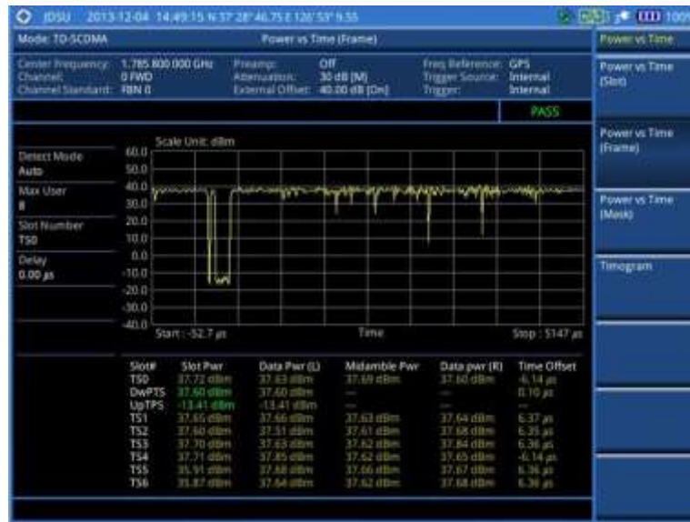
Figure 236 Power vs. time (frame) measurement with TD-SCDMA signal analyzer
