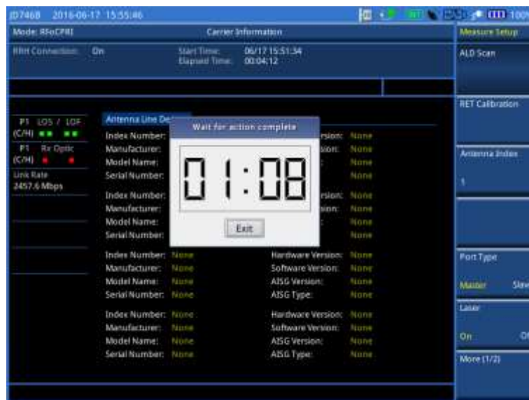
Figure 355 Example of ALD scanning in RET information
