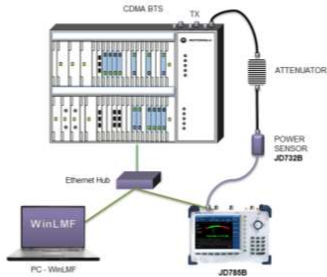
Figure 404 Using external power sensor
