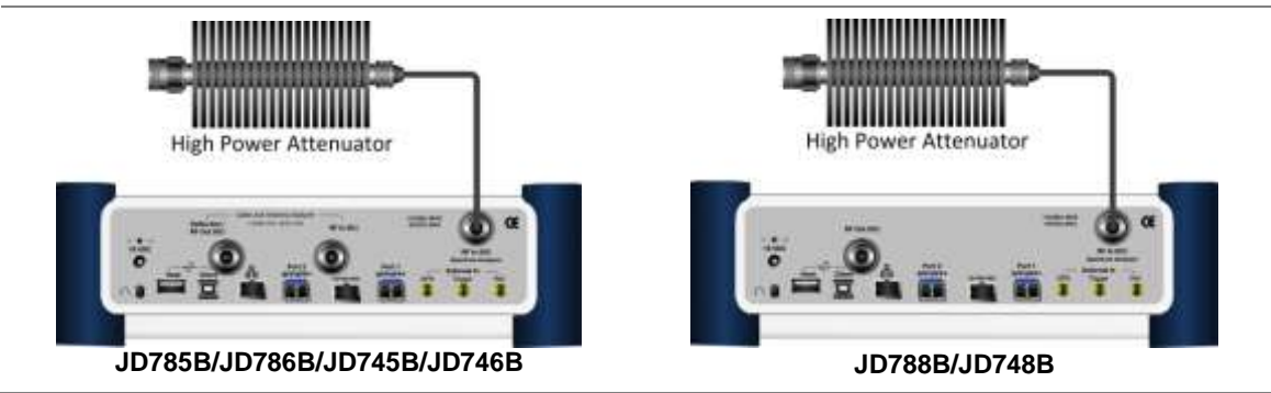
Figure 12 Direct connection
