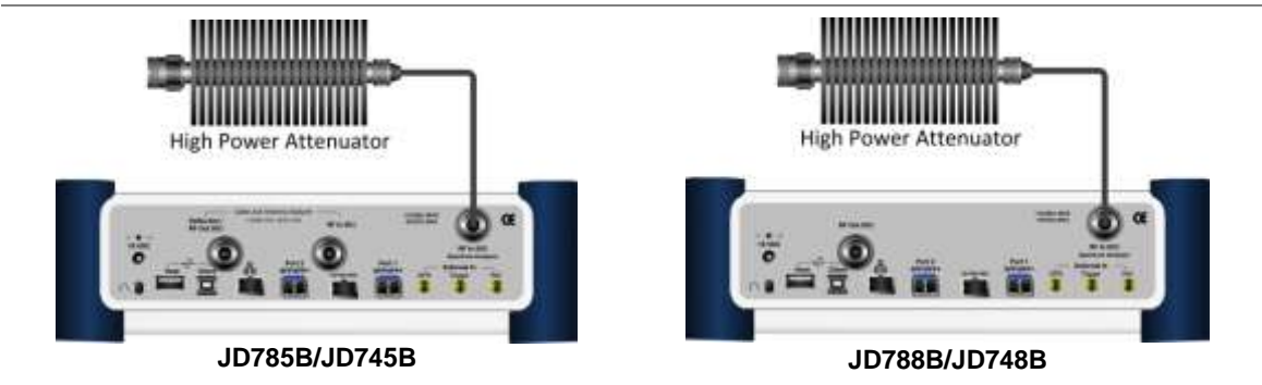
Figure 61 Direct connection
