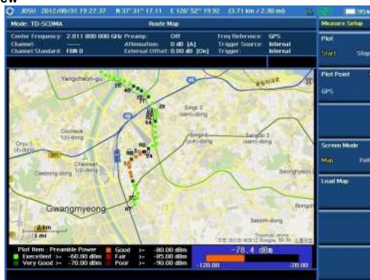
Figure 247 Route map measurement with TD-SCDMA OTA signal analyzer
