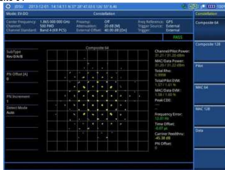
Figure 212 Constellation measurement with EV-DO signal analyzer
