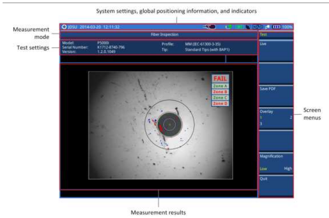
Figure 396 Fiber inspection screen
