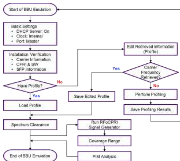
Figure 337 High-level workflow of BBU emulation
