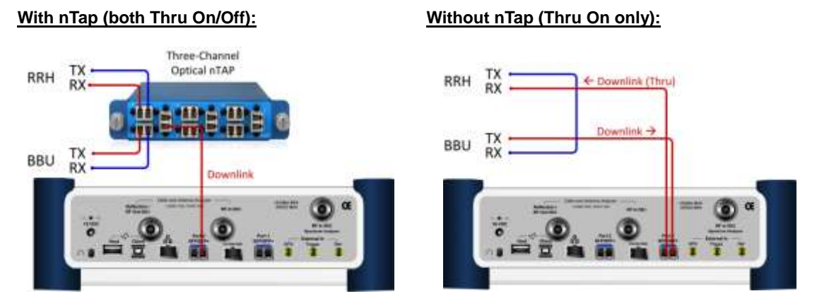
Figure 325 Connection diagram for downlink signal analysis
