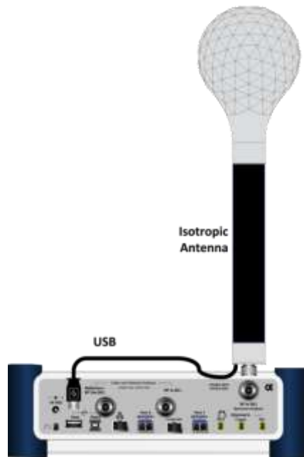
Figure 401 Connection using an isotropic antenna
