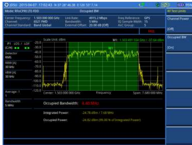
Figure 315 Occupied bandwidth measurement with RFoCPRI LTE-FDD signal analyzer
