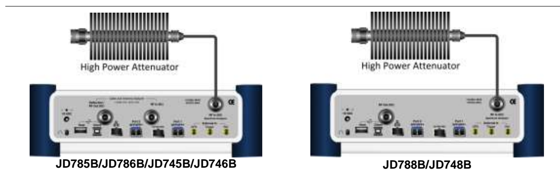
Figure 382 Direct connection
