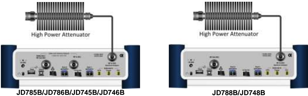
Figure 389 Direct connection
