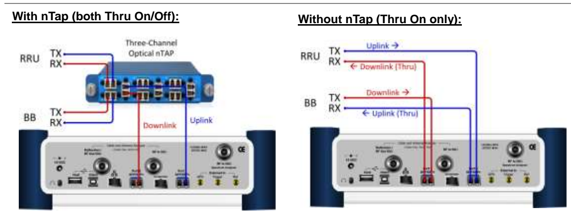
Figure 357 Connection diagram for Layer-2 monitoring mode
