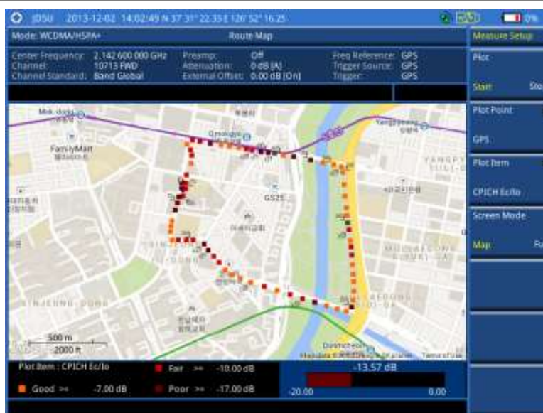
Figure 84 Route map measurement ( CPICH Ec/Io ) with WCDMA/HSPA+ OTA signal analyzer
