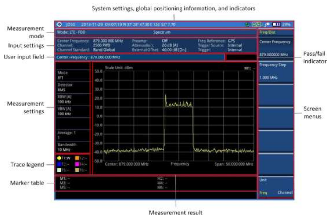
Figure 86 LTE-FDD signal analyzer measurement screen
