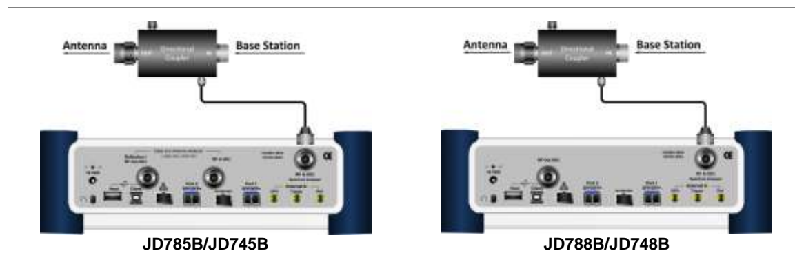
Figure 88 Indirect connection
