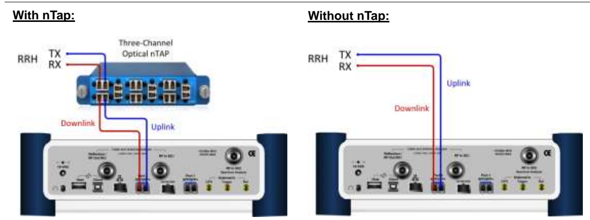
Figure 292 Connection diagram for Layer-2 term testing mode
