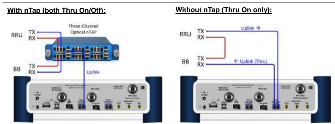
Figure 366 Connection diagram for PIM detection
