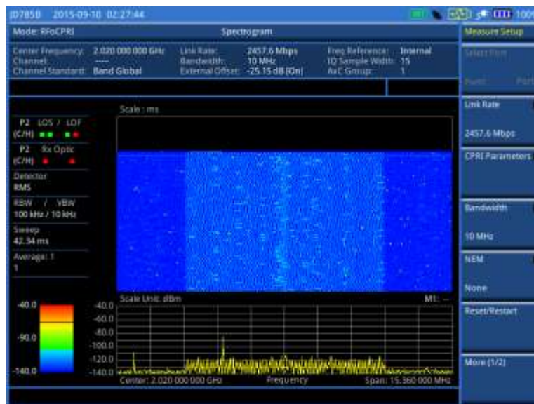
Figure 304 RFoCPRI interference measurement in spectrogram
