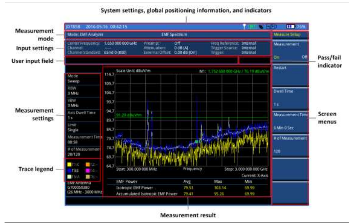
Figure 400 EMF Spectrum measurement screen
