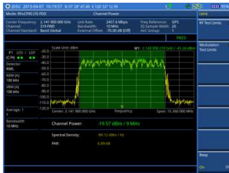
Figure 314 Channel power measurement with RFoCPRI LTE-FDD signal analyzer
