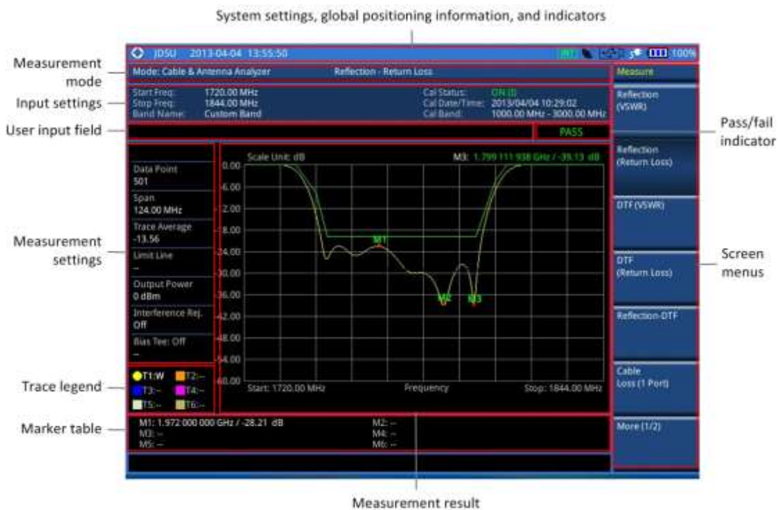
Figure 268 Reflection measurement screen
