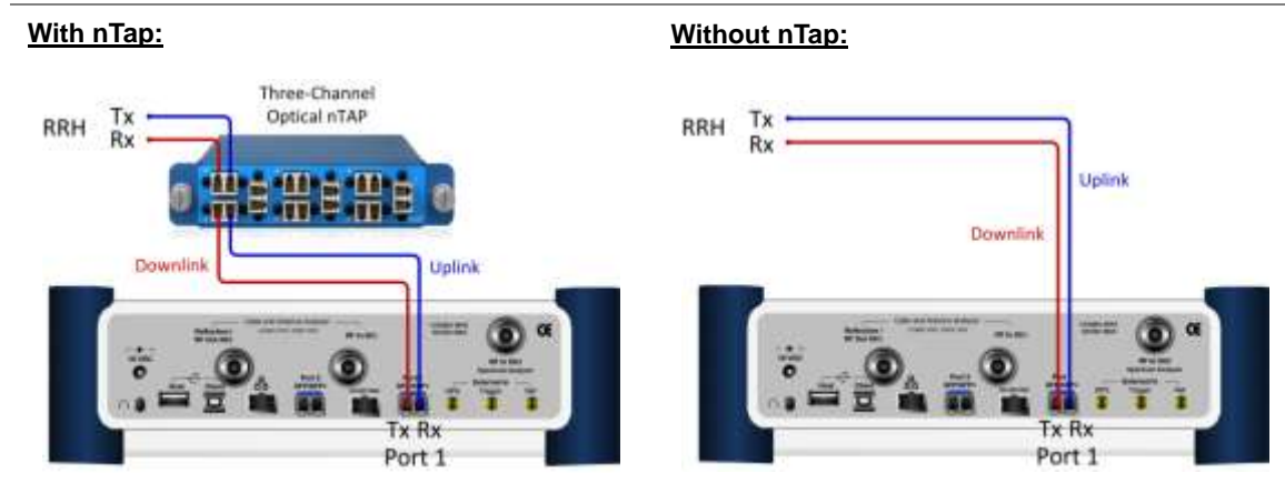
Figure 342 Term mode connection diagram
