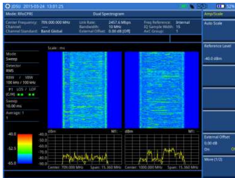
Figure 305 RFoCPRI dual spectrogram analysis
