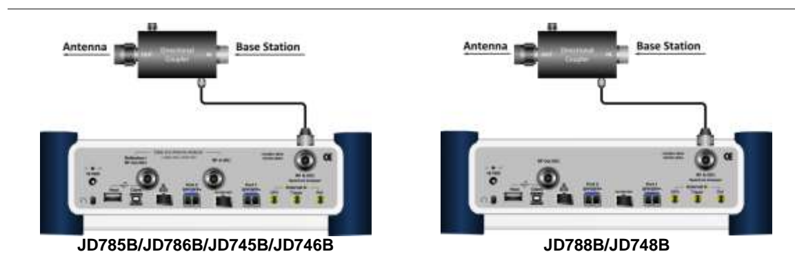
Figure 383 Indirect connection
