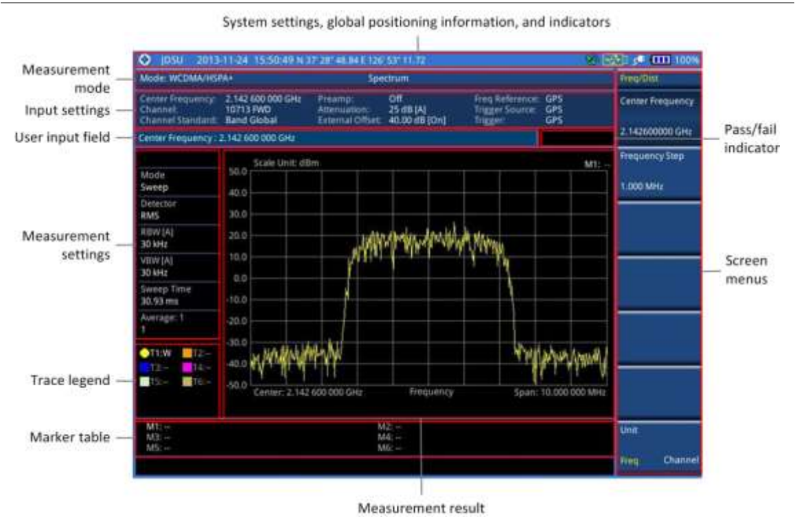
Figure 60 WCDMA/HSPA+ signal analyzer measurement screen
