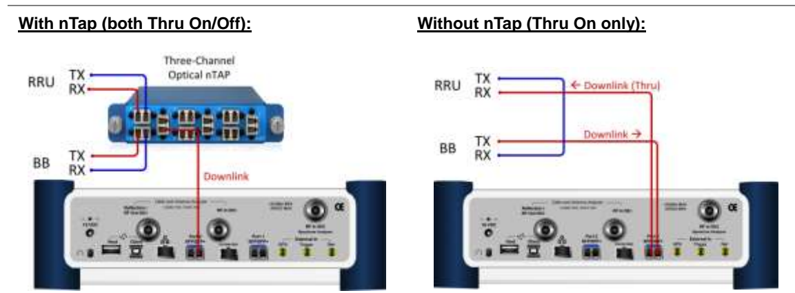
Figure 368 Connection diagram for downlink signal analysis
