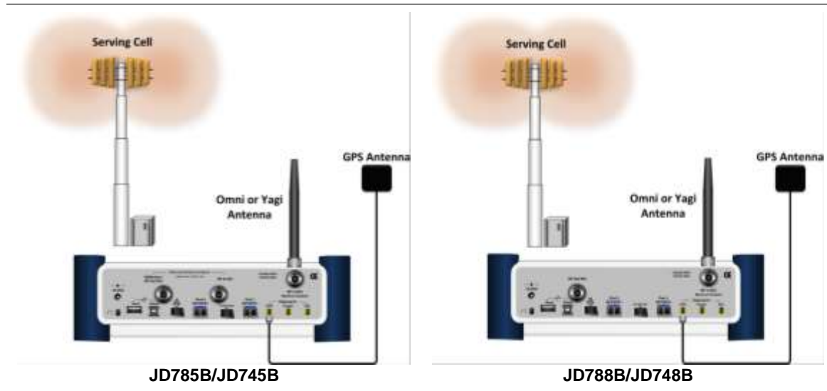
Figure 134 OTA connection
