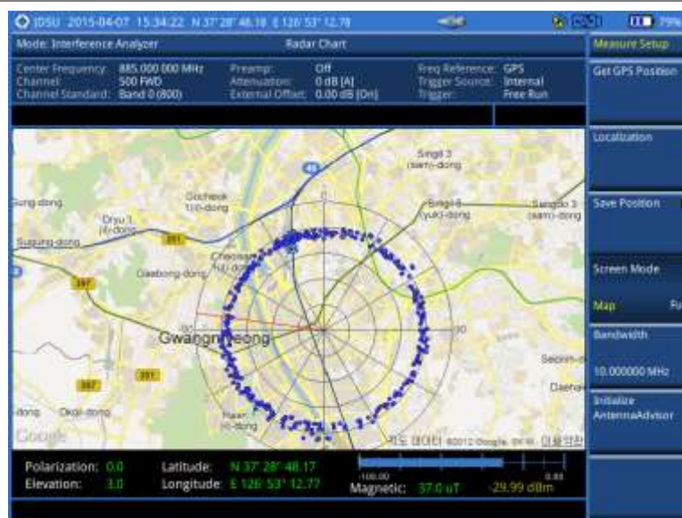
Figure 39 RSSI data plotted on the radar chart
