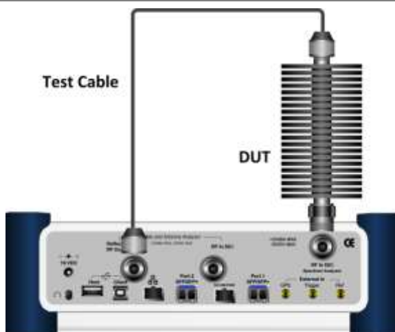
Figure 277 Connection for 2-port scalar measurement
