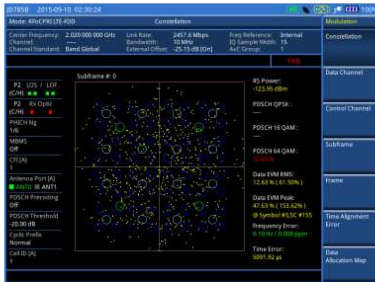
Figure 317 Constellation measurement with RFoCPRI LTE-FDD signal analyzer
