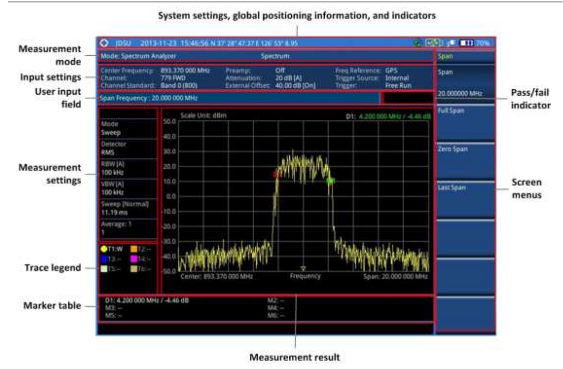
Figure 11 Spectrum measurement screen
