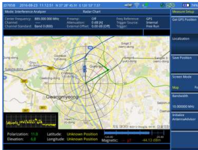
Figure 40 Localized RSSI data on the radar chart
