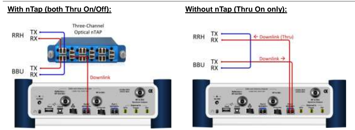
Figure 311 Connection diagram for downlink signal analysis
