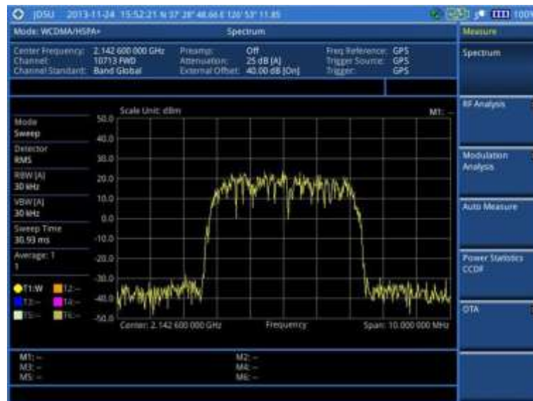
Figure 65 Spectrum measurement screen with WCDMA signal analyzer
