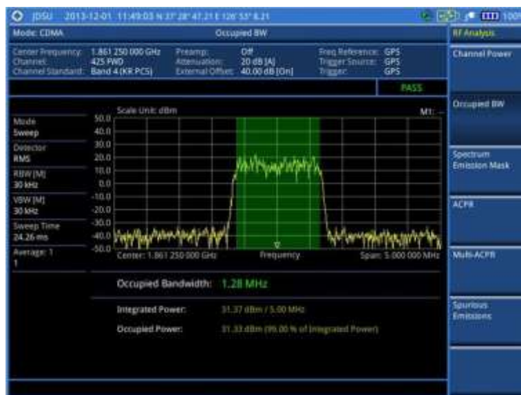
Figure 182 Occupied bandwidth measurement with CDMA signal analyzer
