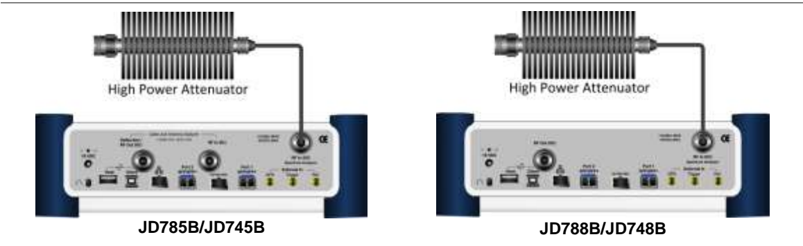
Figure 42 Direct connection
