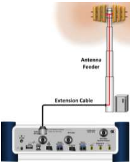
Figure 274 Connection for reflection measurement
