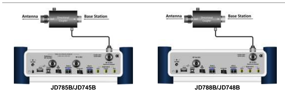
Figure 133 Indirect connection
